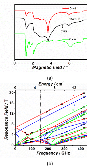
Fig. 3 (a) Typical HF-EPR spectrum of 1 at 154 GHz and 2 K (black) with the simulations using spin Hamiltonian with the true spin S = 3/2 (red: D > 0 ; green: D < 0 ). (b) Resonance field vs. macrowave frequency for EPR transitions for 1 at 2 K. The squares are the experimental points while green, blue and red curves are generated by fitting using program SPIN 33 with the magnetic field parallel to the x , y and z axes of the ZFS tensors, respectively.
