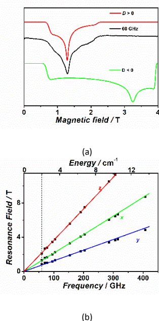
Fig. 4 (a) Typical HFEPR spectrum of 2 at 60 GHz and 2 K (black) with the simulations using spin Hamiltonian with the true spin S = 3/2 (red: D > 0 ; green: D < 0 ). (b) Resonance field vs. macrowave frequency for EPR transitions for 2 at 2 K. The squares are the experimental points while green, blue and red curves are generated by fitting using program SPIN 33 with the magnetic field parallel to the x, y and z axes of the ZFS tensors, respectively.
