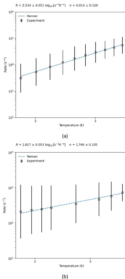
Fig. 7 Plots of relaxation Rates versus T for 1 under 0.15 T (a) and for 2 under 0.1 T (b).
