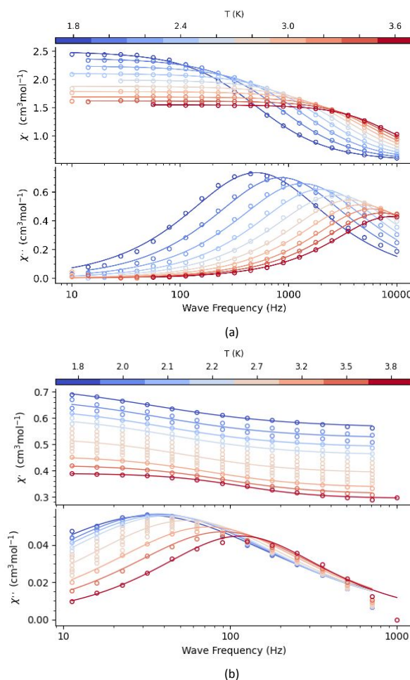
Fig. 5 Frequency dependence of the ac susceptibility from 1.8 K to 3.6 K for 1 (a) at 0.15 T and from 1.8 K to 3.8 K for 2 (b) at 0.1 T, respectively. The solid lines are for eye guide.
