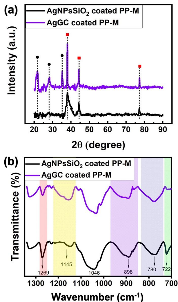
Figure 7. Physicochemical characterization. (a) GLIXRD spectrum (Black circles: cristobalite, red squares: silver) and (b) FTIR spectrum of AgNPsSiO 2 coated PP-M before and after LST with 120 J/cm 2 (AgGC coated PP-M).
