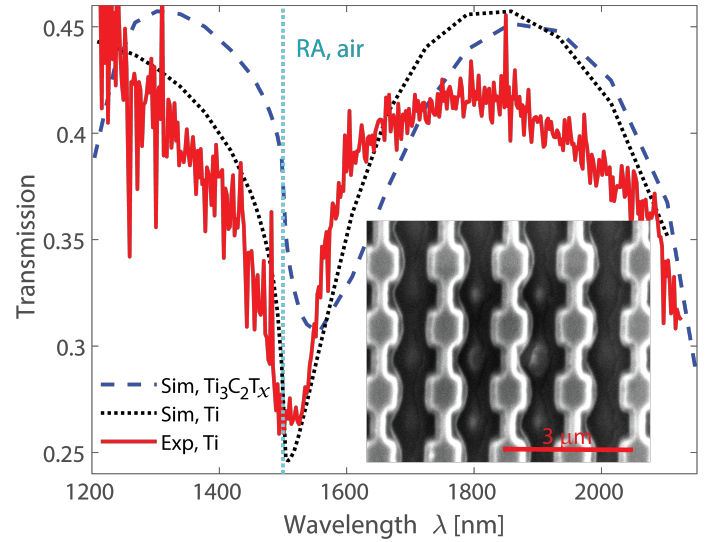
Figure 5: Proof-of-concept experimental characterization of the collective response in the lattice of lossy cuboids. Inset: Scanning electron microscope image of the fabricated metasurface. Antennas have a cuboid shape with a_x = a_y = 600 nm, a_z = 400 nm, and bridge width w = 200 nm. Notations ‘Sim’ and ‘Exp’ correspond to the numerical simulation and experimental measurement, respectively. The metasurface is fabricated on a fused silica substrate. The metasurface is illuminated with the y-polarized light. The antennas are arranged into a periodic lattice with periods D_x = D_y = 1500 nm. The solid cyan line ‘RA, air’ denotes the Rayleigh anomaly in the free space ( \lambda_{RA,air} = D_{x,y} ).
