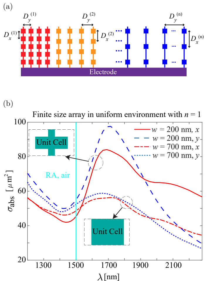
Figure 6: a Schematic of the resonant electrode of a two-dimensional multiple-period interconnected array of the MXene antennas. Each color represents a patch with a distinct pitch based on periodicities of D_x^{(n)} and D_y^{(n)} from 1 to n . This electrode enables enhanced photoemission across a broad spectrum of wavelengths. b Resonant excitations in finite-size array consisting of the 7 \times 7 = 49 interconnected MXene antennas. We consider MXene antennas of cube shape with a_x = a_y = a_z = 700 nm connected with ‘bridges’ with the width of w = 200 nm or 700 nm. The latter corresponds to the continuous stripes. Notations ‘x’ and ‘y’ correspond to the illumination of light with x- or y-polarization (see Figure 1c ). The cuboids are placed into a regular array with pitches D_y = D_x = 1500 nm. Antennas are in the uniform surrounding with n = 1 . The absorption cross-section spectra are obtained with full-wave numerical simulations. The solid cyan line denotes the Rayleigh anomaly wavelengths: ‘RA, air’ denotes the Rayleigh anomaly in the free space ( \lambda_{\text{RA,air}} = D_{x,y} ).
