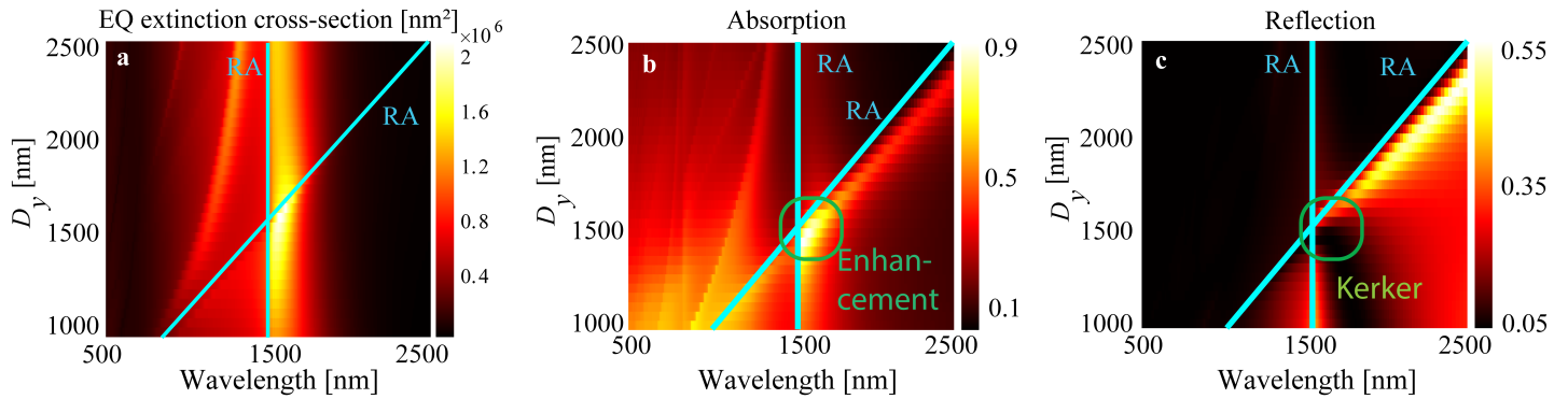
Figure 2: Resonance response in the MXene-scatterer lattice: a EQ extinction cross-section, b Absorption, and c Reflection. The data are acquired through the comprehensive numerical simulations of sphere antennas within the rectangular lattice. The results are shown for the changes in D_y and constant D_x = 1500 nm. The surrounding environment is free space with n = 1 . The solid cyan lines ‘RA’ denote the Rayleigh anomaly wavelength in the free space ( \lambda_{RA} = D_{x,y} ). The sphere’s size is R = 450 nm. Green circles denote the regions of enhanced absorption and generalized lattice Kerker effect in panels b and c , respectively.
