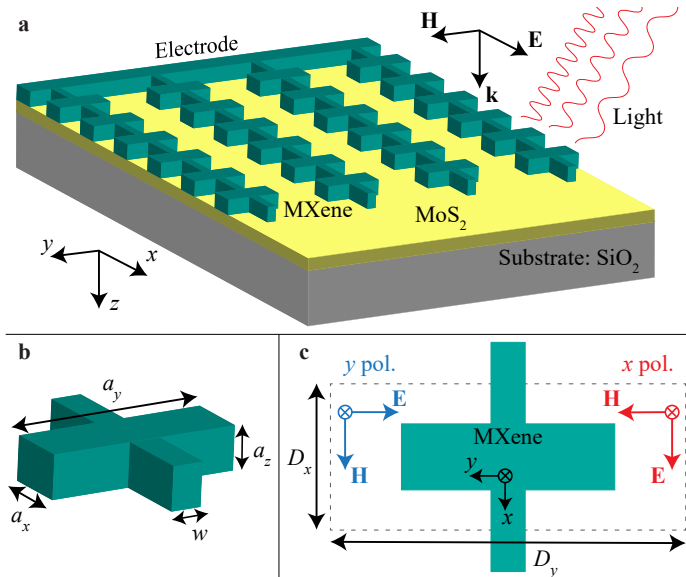
Figure 1: a Electrode schematic: MXene ( \text{Ti}_3\text{C}_2\text{T}_x ) resonant antennas (dark green) on the few-layer \text{MoS}_2 (yellow) and the silica substrate (grey). The antennas are interconnected by the ‘bridge’ and attached to the electrode strip at one end, thus forming a metasurface. b Schematic of an array unit cell with MXene antenna considered in the numerical simulations. The dimensions of the cuboid particle are a_x , a_y , and a_z . c Top view of the unit cell simulated under two different light polarizations: the red arrows are for the x -polarization, and the blue arrows are for the y -polarization. D_x and D_y are the periodicities in the x - and y -directions, respectively. The ‘bridge’ connects metasurface antennas in the x -direction and has width w in the y -direction.
