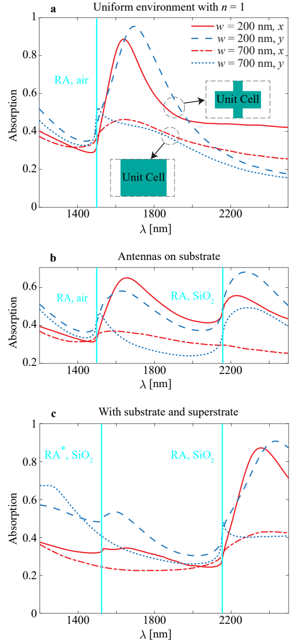
Figure 3: Light absorption as a contribution to the volume mechanism of the hot-electron generation through resonant excitations in the interconnected MXene antennas arranged in the periodic array (metasurface): a Antennas in the uniform surrounding with n = 1 , b on a few-layer MoS 2 and SiO 2 substrate, and c on a few-layer MoS 2 and SiO 2 substrate with an index-matching superstrate. We consider MXene antennas of cube shape with a_x = a_y = a_z = 700 nm connected with ‘bridges’ with the width of w = 200 nm or 700 nm. The latter corresponds to the continuous stripes. Notations ‘ x ’ and ‘ y ’ correspond to the illumination of light with the x - or y -polarization (see Figure 1c). The antennas are arranged into a periodic lattice with periods D_x = D_y = 1500 nm. The solid cyan lines denote the Rayleigh anomaly wavelengths: ‘RA, air’ denotes the Rayleigh anomaly in the free space ( \lambda_{\text{RA,air}} = D_{x,y} ), and ‘RA, SiO 2 ’ denotes the Rayleigh anomaly in SiO 2 ( \lambda_{\text{RA,SiO}_2} = n_{\text{SiO}_2} D_{x,y} ), correspondingly. ‘RA*, SiO 2 ’ denotes a next-order Rayleigh anomaly at \lambda_{\text{RA}^*} = n_{\text{SiO}_2} D_{x,y} / \sqrt{2} .
