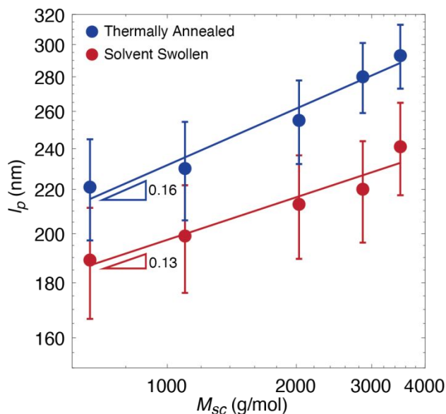
Figure 2: Persistence lengths of PMMA bottlebrush polymers in non-swollen and 20% toluene-swollen linear PMMA films as a function of side chain molecular weight. Each data point consists of 350 chains. Error bars are 90% confidence intervals, which were determined by calculating the standard deviation in l_p based on 10 sets of 350 wormlike chains from simulation (see previous work for details). 22,23 Lines represent power law fits. Due to uncertainties in our technique, we are less confident in lower l_p values. Fitting the highest three points of the solvent-swollen series results in a scaling exponent of 0.22. Note that the data spans less than one decade in the abscissa, so we encourage caution in interpreting the power law fit in general.
