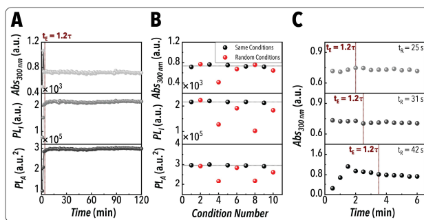
Figure 3. Characterization of the developed flow chemistry platform performance for continuous operation and successful/reproducible synthesis of Pb-free MHP NCs: A) Temporal evolution of Abs_{300\text{ nm}} , PL_I , and PL_A for a specific synthesis condition over 120 min. B) Assessment of the developed flow chemistry platform synthesis reproducibility by utilizing an experimental perturbation study. C) Examination of the impact of dynamic residence time to determine the number of residence times (equilibrium time) applicable to all autonomous conditions.
