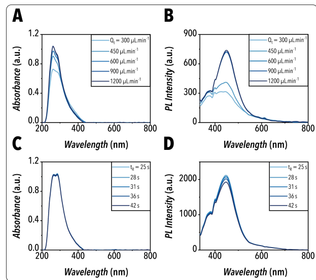
Figure 4. In-flow screening for: The effect of total volumetric flowrate on the in-situ recorded A) absorption and B) PL spectra while utilizing the same reaction time. The effect of reaction time on the in-situ recorded C) absorption and D) PL spectra while utilizing total flowrates above 600 \mu\text{L}/\text{min} to ensure the reaction mixing-independency.
