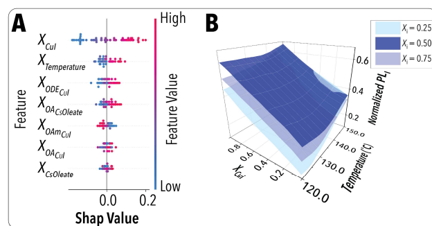
Figure 7. Accelerated fundamental studies of Cs_3Cu_2I_5 NCs synthetic chemistry using the digital twin model: A) Shapley additive explanation plot of PL_1 . B) Surface plot showing the impact of the top two synthesis input parameters on PL_1 .
