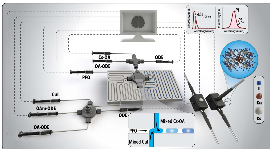
Figure 2. Schematic illustration of the developed SDFL for fast-tracked synthesis and development of Pb-free MHP NCs.
