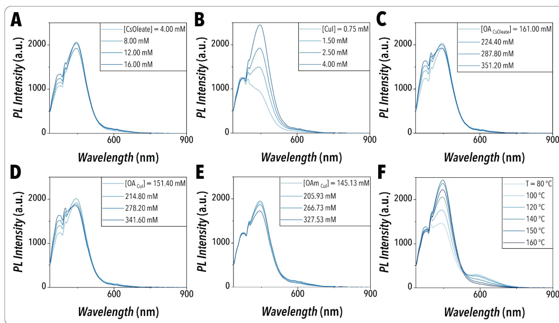
Figure 5. In-situ recorded UV-Vis PL spectra of the partial grid search on the input synthesis parameters, including A) [CsOleate], B) [CuI], C) [OAcCsOleate], D) [OAcCuI], E) [OAmCuI], and F) reaction temperature, while maintaining the reaction time constant. The complete list of experimental conditions used for the partial grid search study is provided in Table S1 .
