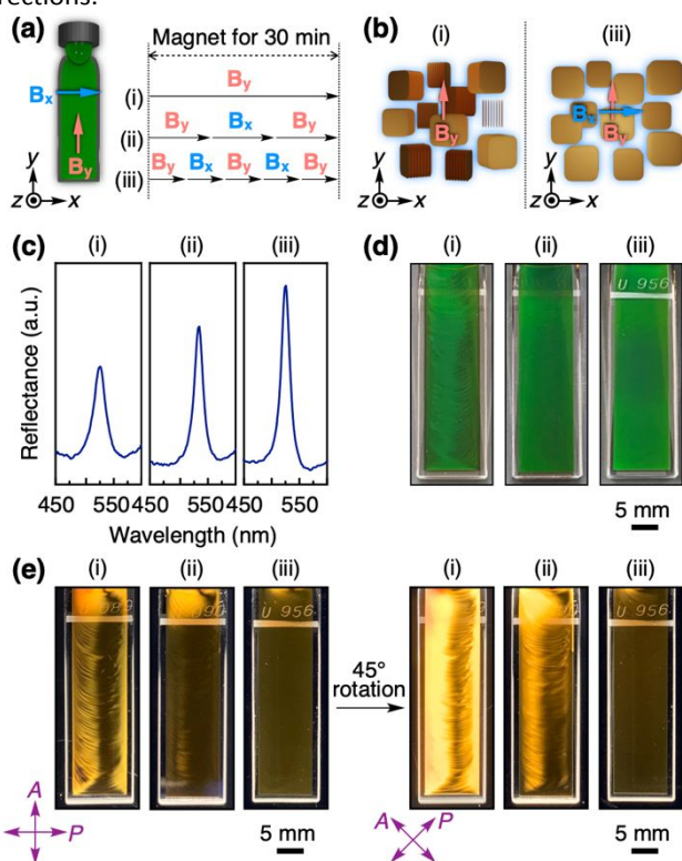
Fig. 5 (a) Magnetic application processes (i–iii) for improving the quality of a structural color. A 12 T magnetic field is alternately applied along the y - and x -axis directions with a total magnetic application time of 30 min at 50 °C. (b) Schematic illustrations of the orientation of GO nanosheets after processes (i) and (iii). (c) Reflection spectra, (d) optical images, and (e) polarized optical images of a photonic crystal of GO nanosheets ([GO] = 0.3 wt%) after processes (i–iii).
