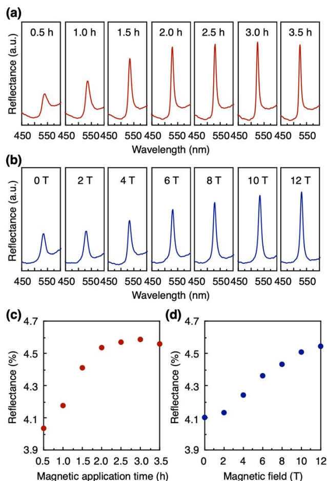
Fig. 4 (a–d) Reflection spectra (a,b) and plots of peak intensity in the spectra (c,d) as a function of the application time of a 12 T magnetic field at 50 °C (a,c) and the magnetic strength with an application time of 3 h (b,d) using a photonic crystal of GO nanosheets ([GO] = 0.3 wt%) with the magnetic treatment along the y -axis.
