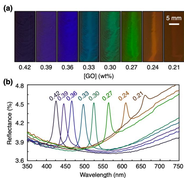
Fig. 3 (a) Optical images and (b) corresponding reflection spectra of photonic crystals of GO nanosheets with different concentrations ([GO] = 0.21–0.42 wt%) after the magnetic treatment along the y -axis.
