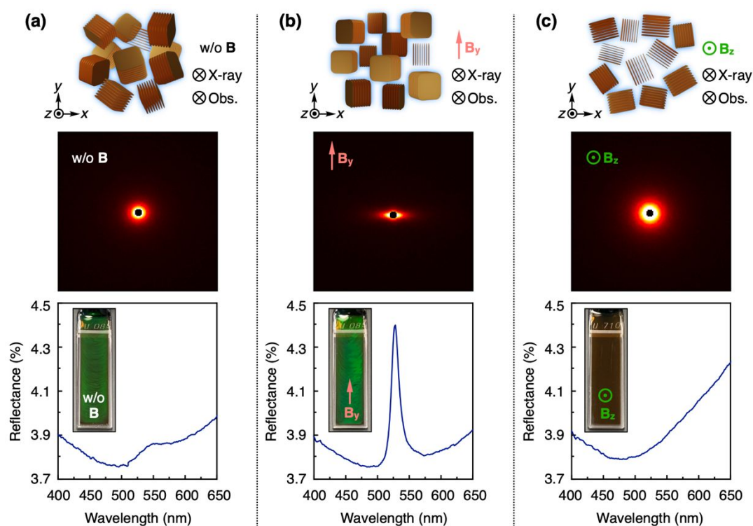
Fig. 2 (a–c) Schematic illustrations of the orientation of GO nanosheets and 2D SAXS profiles of gel samples of GO nanosheets ([GO] = 0.1 wt%) fixed by photo-polymerization of acrylic monomers and crosslinkers (upper) and reflection spectra (lower) with optical images (inset) of photonic crystals of GO nanosheets ([GO] = 0.3 wt%) prepared without a magnetic application (a) and with a 12 T magnetic application along the y-axis (b) and z-axis (c).
