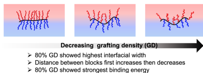
Scheme 3. Schematic illustration of interfacial conformation of JBCP compatibilizers with variable grafting densities for N_{BB}=100 .
