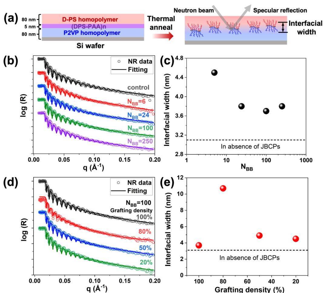
Figure 2. (a) Schematic illustration of probing interfacial width from neutron reflectivity (NR); (b) NR of DPS || (DPS-PAA) n || P2VP || Si for different N_{BB} of JBCPs. The NR profiles are shifted for clarity. (c) Interfacial width between PS and P2VP homopolymer in presence of JBCPs of variable N_{BB} at 100% GD. (d) Neutron reflectivity (NR) of DPS || (DPS-PAA) n || P2VP || Si for different GD values at N_{BB}=100 . The NR profiles are shifted for clarity. (e) Interfacial width between PS and P2VP homopolymer in presence of JBCPs with variation of grafting density at N_{BB}=100 .
