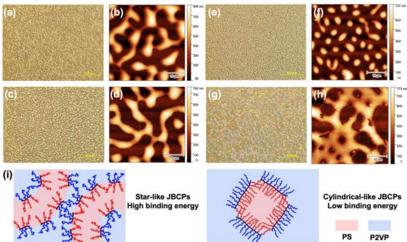
Figure 7. Morphologies of thin film blends contained PS homopolymer and P2VP homopolymer (70 wt.% to 30 wt.%) with 10 wt.% JBCP additives of different N_{BB} . GD=100% for all N_{BB} . POM images of (a) N_{BB}=6 , (c) N_{BB}=24 , (e) N_{BB}=100 , and (g) N_{BB}=250 . AFM images of (b) N_{BB}=6 , (d) N_{BB}=24 , (f) N_{BB}=100 , and (h) N_{BB}=250 . (i) Schematic illustration of N_{BB} effect on binding energy at homopolymer interfaces. P2VP domain was washed by ethanol after thermal annealing of thin film blends.
