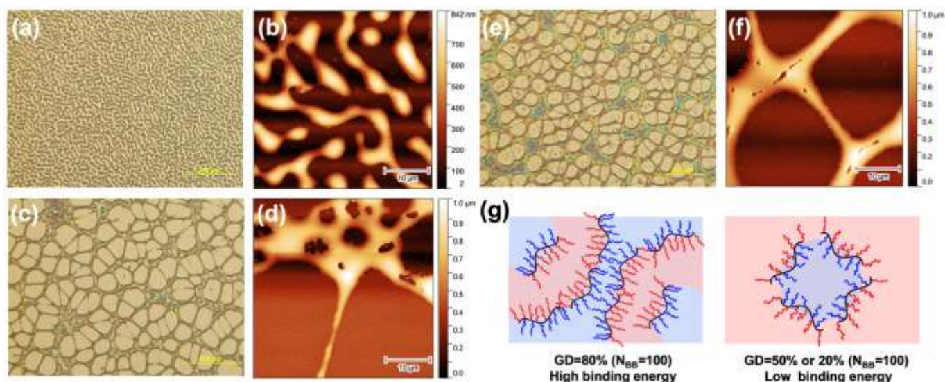
Figure 8. Morphologies of thin film blends containing PS homopolymer and P2VP homopolymer (70 wt.% to 30 wt.%) with 10 wt.% JBCP for different grafting densities at N_{BB}=100 . POM images of grafting density (a) 80%, (c) 50%, and (e) 20%. AFM images of (b) 80%, (d) 50%, and (f) 20%. (g) Schematic illustration of grafting density effect on binding energy at homopolymer interfaces. P2VP domain was washed by ethanol after thermal annealing of thin film blends.
