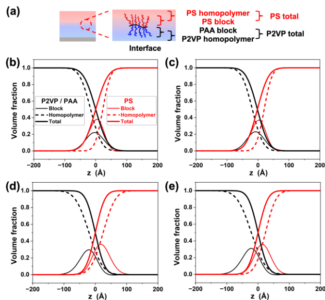
Figure 3. (a) Schematic illustration of a JBCP at polymer-polymer interface. Volume fraction profiles of different components at interfaces for JBCPs with variation of N_{BB} , (b) N_{BB}=6 , (c) N_{BB}=24 , (d) N_{BB}=100 , and (e) N_{BB}=250 . z is the distance in Angstrom from the homopolymer interface. The legends for (c)-(e) are same as (b).
