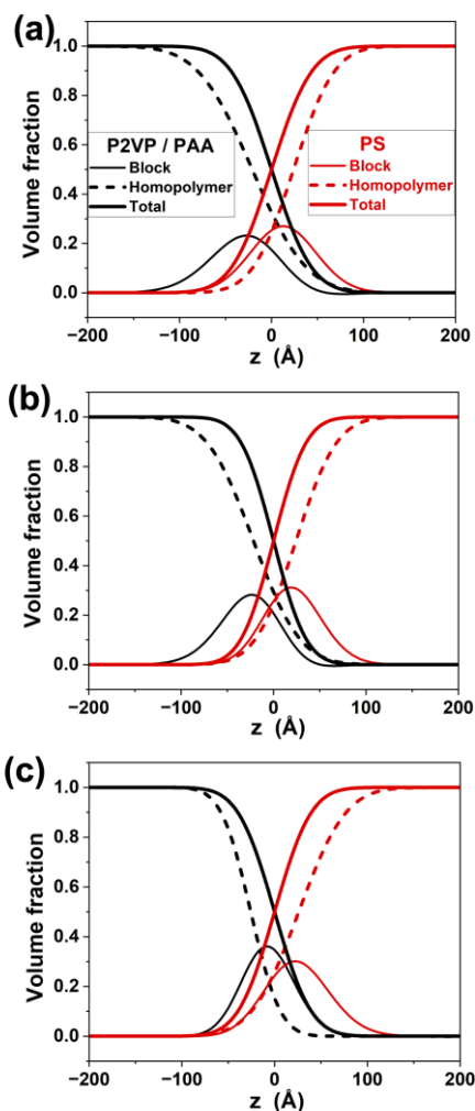
Figure 5. Volume fraction profiles of different components at interfaces for JBCPs with N_{BB}=100 at different grafting densities of (a) 80%, (b) 50%, and (c) 20%. z is the distance from the homopolymer interface. The legends for (b) and (c) are same as (a).
