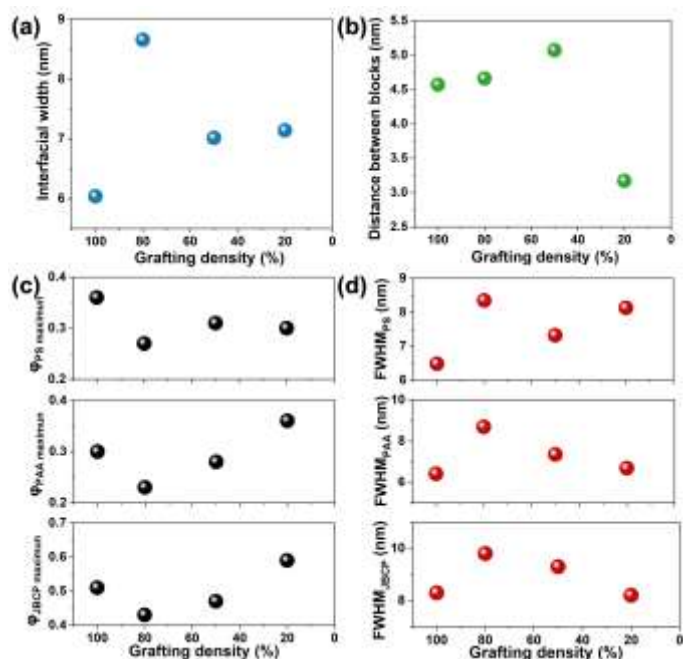
Figure 6. Characteristics of segment density distributions for different grafting densities (GD) with N_{BB}=100 . (a) Interfacial width solved from PS || (DPS-PAA) n || DP2VP || Si. (b) Distance ( d ) between two blocks (c) Volume fraction maximum ( \phi_{maximum} ) of PS block, PAA block and JBCP molecule. (d) Full-width half maximum (FWHM) of PS block, PAA block and JBCP molecule.
