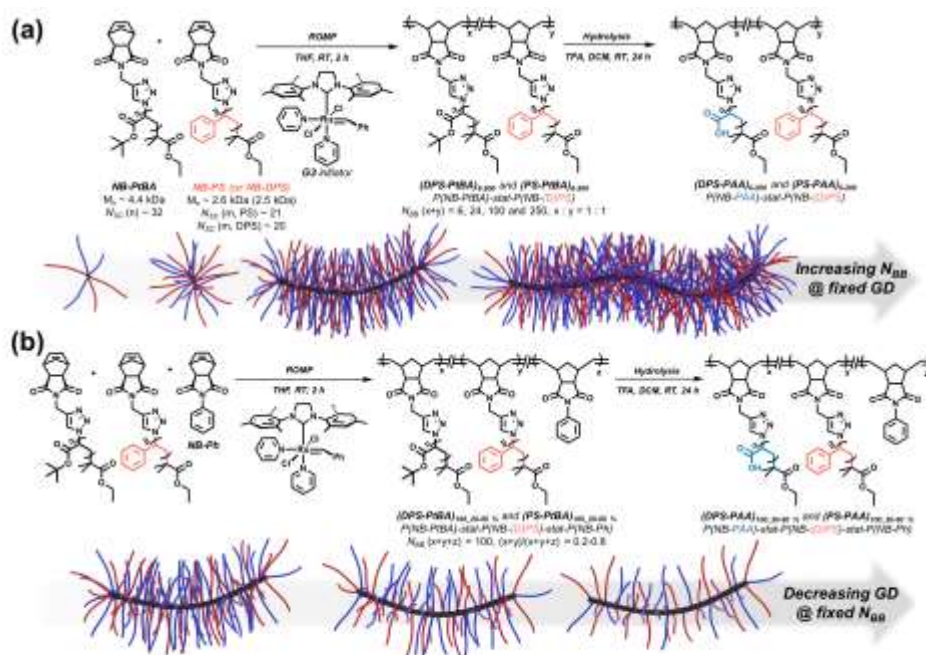
Figure 1. (a) ROPM of NB-PtBA and NB-DPS/PS, and subsequent acid-catalyzed hydrolysis of t -BA repeating units. Illustrations of polymer shapes as a function of N_{BB} . (b) ROPM of NB-PtBA, NB-DPS/PS, and NB-Ph, and subsequent acid-catalyzed hydrolysis of t -BA repeating units. Illustrations of polymer shapes as a function of GD. PS is shown as example in scheme.
