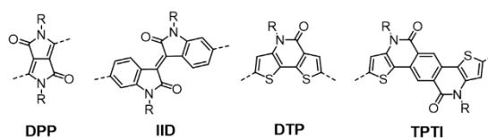
Fig. 1 Representative lactam-containing \pi -systems.
