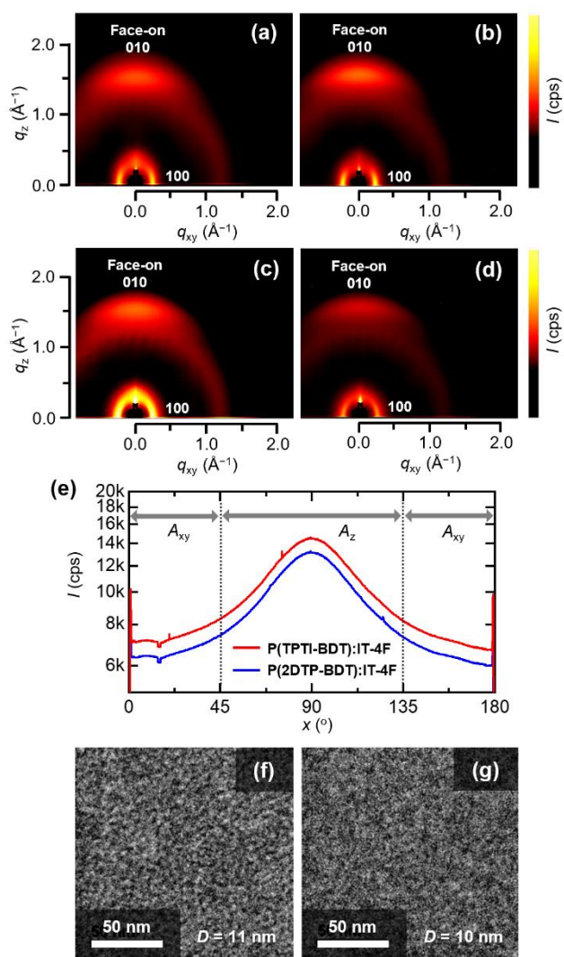
Fig. 5 Two-dimensional GIXD images for (a) P(TPTI-BDT) and (b) P(2DTP-BDT) neat films and (c) P(TPTI-BDT):IT-4F (1:1, w/w) and (d) P(2DTP-BDT):IT-4F (1:1, w/w) blend films. (e) Pole figures for the \pi - \pi stacking diffractions ( d = 4.25 – 2.88 Å) in the blend films. TEM images of (f) P(TPTI-BDT):IT-4F (1:1, w/w) and (g) P(2DTP-BDT):IT-4F (1:1, w/w) blend films. The D values represent the average domain sizes calculated by 2D FFT analysis.
