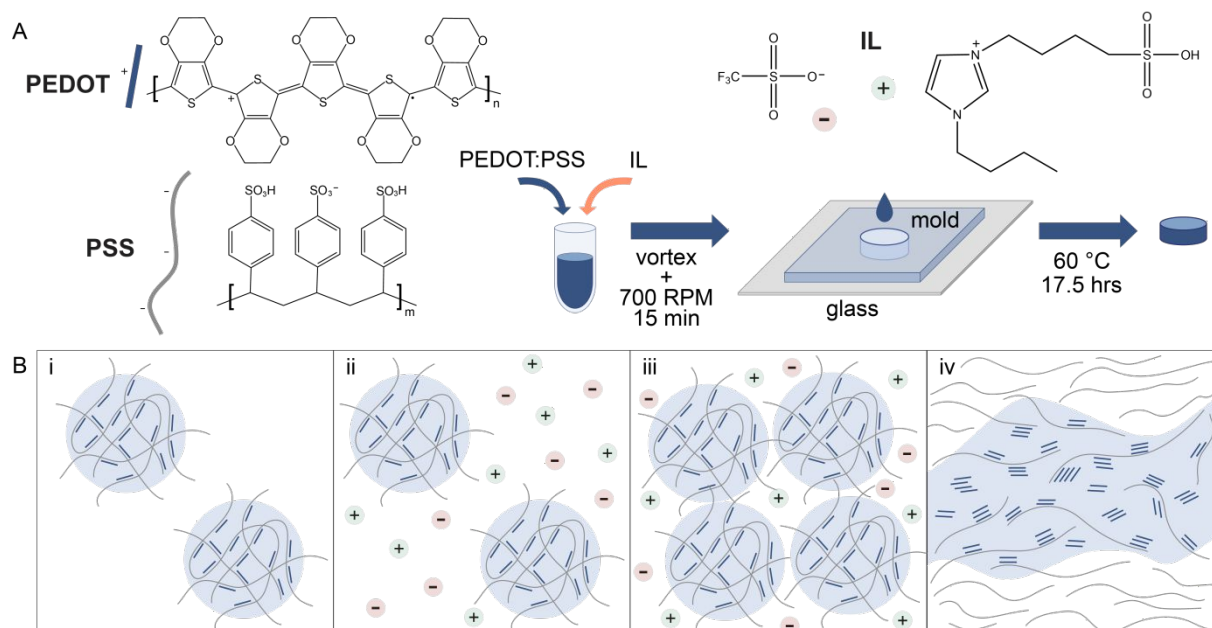
Figure 1. Schematic of PEDOT:PSS-IL hydrogel fabrication and gelation mechanism.
