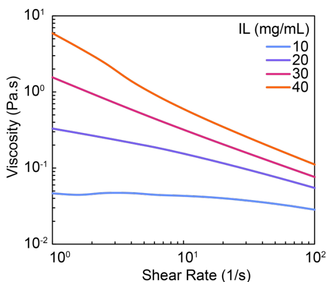
Figure 3. Increasing ionic liquid concentration increases viscosity of liquid-phase PEDOT:PSS-IL mixtures. All liquid-phase hydrogel precursor mixtures are shear-thinning. Representative plots of viscosity as a function of shear rate measured 20 minutes after IL addition to PEDOT:PSS dispersion.
