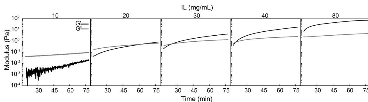
Figure 2. Ionic liquid concentration affects gelation kinetics of PEDOT:PSS hydrogels. Oscillatory rheology over time to measure G' and G'' , storage and loss modulus, respectively (representative plots). The transition from liquid to gel ( G' - G'' cross-over), was captured for mixtures containing 20, 30, and 40 mg/mL IL over approximately 75 minutes. As the IL concentration increases, the time to G' - G'' cross-over shortened. At 10 mg/mL IL, the mixture remained a liquid over the time of study, while 80 mg/mL was already a gel. PEDOT:PSS-IL mixtures were stirred for 15 min prior to addition to the rheometer, and thus, the x axis represents time of mixture preparation (after IL addition).
