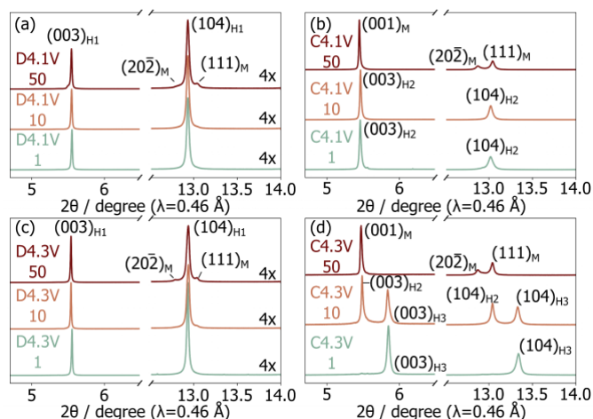
Fig. 2 Selected regions from the synchrotron XRD patterns collected on ex situ samples in the (a,c) discharged and (b,d) charged states for cells cycled up to (a,b) 4.1 V and (c,d) 4.3V. Crystallographic parameters derived from the refinements are tabulated in Table S1 and full synchrotron XRD patterns are provided in Fig. S3–6.
