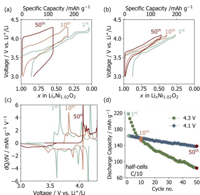
Fig. 1 Electrochemical data for LiNiO 2 /Li half cells cycled at a rate of C/10 (C=200mAh -1 ). Voltage profiles for selected cycles are shown for the (a) 4.3 V and (b) 4.1 V upper cut-off voltage. (c) differential capacity, dQ/dV (mAh g -1 V -1 ), plot for a cell cycled to 4.3 V. (d) The average discharge capacity of three cells cycled up to 4.3 V or 4.1 V over 50 cycles. angle spinning probe (MAS). Our results allow us to determine for the first time the structure and Li content of the fatigued domains, as well as the nature of the defects, arising in LNO particles during extended cycling.
