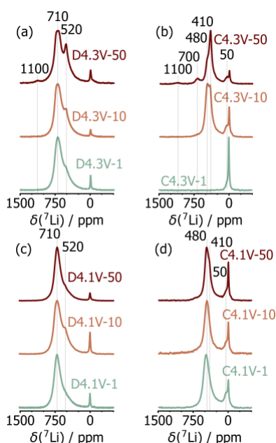
Fig. 3 ^7\text{Li} solid-state NMR spectra collected on ex situ samples in the (a,c) discharged and (b,d) charged states for cells cycled to (a,b) 4.3 V and (c,d) 4.1 V. All spectra were acquired at 2.35 T and 60 kHz MAS and are normalized to the most intense signal.
