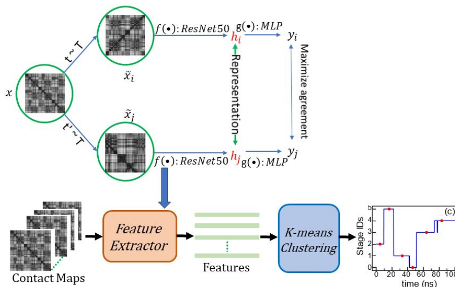
Fig. 1. The framework of contrastive learning contact map feature extraction and protein structure transition stage detection. (\tilde{x}_i, \tilde{x}_j) are considered a positive pair when they represent correlated views of the same contact map x , produced through stochastic data augmentations t \sim T and t' \sim T , respectively. The augmentation sequence T , employed in this study, is executed sequentially and applied randomly with a 0.5 probability, encompassing random cropping followed by resizing back to the original dimensions, Sobel filtering, random horizontal flipping, and Gaussian blurring. The backbone representation encoder, denoted as f(\cdot) , specifically employs Resnet50. g(\cdot) , a compact projection head, is designed as a multilayer perceptron (MLP) featuring a single hidden layer. Both f(\cdot) and g(\cdot) are trained with the primary objective of maximizing agreement among positive pairs of augmented contact map views using the loss function outlined in Eq. (1). The feature extractor, obtained via contrastive learning, processes the contact maps. Subsequently, the k -means clustering algorithm is used to group the series of contact maps into stages representing structural transitions.
