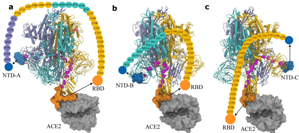
Fig. 6. Pathway of the allosteric regulation in the spike protein obtained via Ohm from (a) NTD-A, (b) NTD-B, and (c) NTD-C, to the RBD on subunit C. NTDs are colored in dark blue. The other color codes are the same as those in Fig. 5. The corresponding rotation movies are provided as ESI Movie S2.
