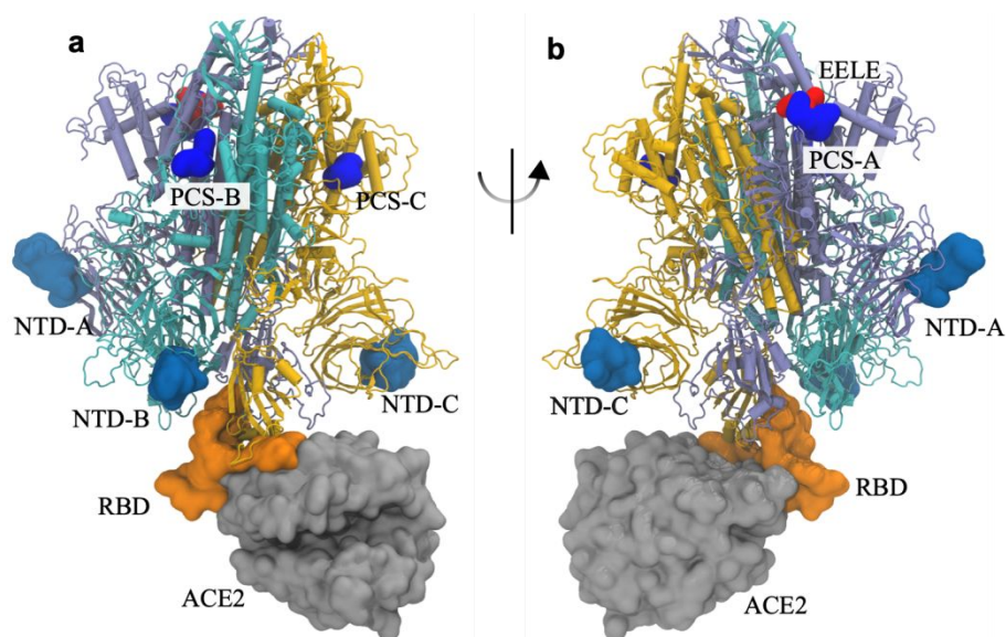
Fig. 2. Molecular structure of the spike-ACE2 complex in the presence of the neutralizing tetrapeptides EELE. (a) Front view and (b) back view. The three subunits of the trimeric spike protein are colored in ice blue/cyan/orange for the subunits A/B/C, respectively. The spike protein's PCS, NTD, and RBD are colored in blue, dark blue, and orange, respectively. The ACE2 receptor and the tetrapeptide EELE are colored in silver and red, respectively.
