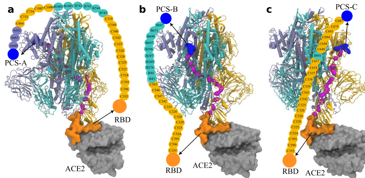
Fig. 5. Pathway of the allosteric regulation in the spike protein obtained via Ohm from (a) PCS-A, (b) PCS-B, and (c) PCS-C, to the RBD on subunit C. The three subunits of the trimeric spike protein are colored in ice blue/cyan/orange for the subunits A/B/C, respectively. PCSs are colored in blue and the RBD on subunit C in orange, which is in direct contact with ACE2 (in silver). The backbone atoms on the connecting amino acids are indicated by magenta; the names of the connecting amino acids are provided in the illustration. The corresponding rotation movies are provided as ESI Movie S1.
