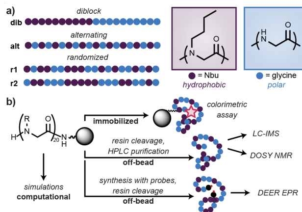
Figure 2. Sequence workflow and design. a) Schematic describing the 20mer peptidomimetics with identical compositions (left) and monomer structures (right): hydrophobic (N-butylglycine) and polar (glycine). b) Schematic describing use of solid-phase synthesis to prepare 20mers for characterization of disorder.
