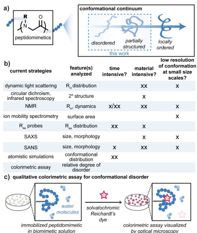
Figure 1. Overview of the continuum of disorder for peptidomimetics and methods for structural characterization. a) Scope of structural disorder of sequence-defined oligomers. b) Existing methods for characterizing oligomers, where R_{\text{ee}} denotes the end-to-end distance of the chain. Time intensive techniques typically require > 20 min (X), > 2 h (XX); material intensive typically require > 10 \mu\text{g} (X), > 0.5 mg (XX); and small size scales refers to materials smaller than 3 kDa. c) Schematic of the colorimetric platform for characterizing
