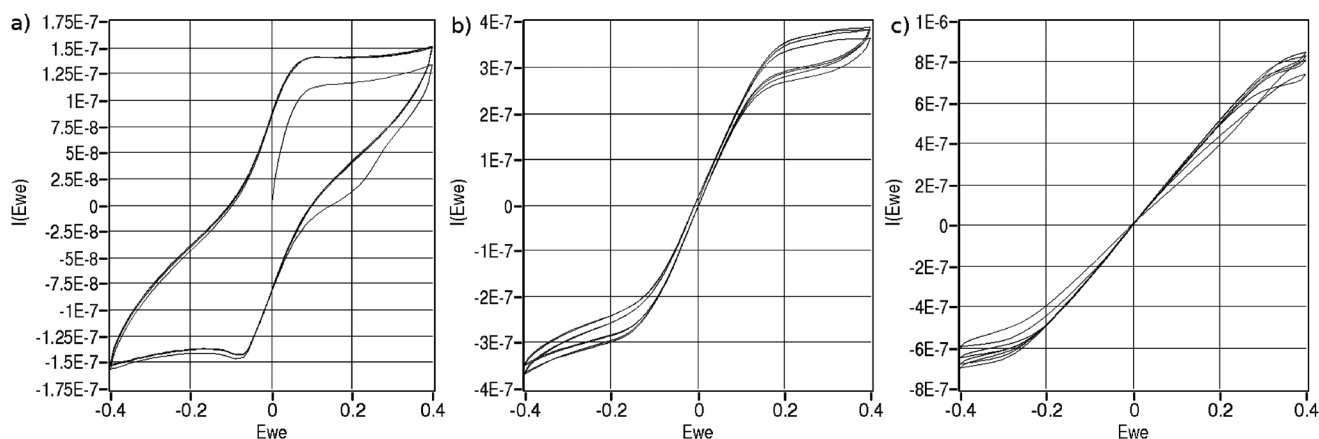
Fig. 6 Cyclic voltammograms recorded in a solution containing 2.5 mM ferrocyanide, 2.5 mM ferricyanide, 0.1 M \text{KNO}_3 and 2 mM phosphate buffer using a chip with a working electrode area of 2.4 mm 2 . Scan rate was 20 mV/s. a) no-flow, b) 0.1 \mu\text{L}/\text{min} c) 0.25 \mu\text{L}/\text{min} .
