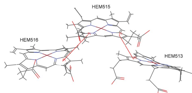
Fig. 3 Details of the interactions linking the three porphyrins of the cytochrome c -552 from Wolinella succinogenes (PDB ID code 3bnj). The \pi - \pi interactions are marked with red lines (HEM513:D—HEM515:D, HEM515:A—HEM516:A).
