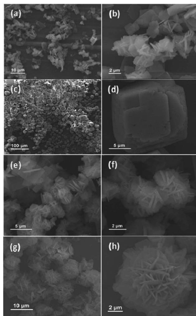
Fig. 1 SEM images of the synthesized NiCo 2 O 4 samples from different hydrothermal reaction times: (a–b) 3 h; (c–d) 6 h; (e–f) 9 h; (g–h) 12 h.
