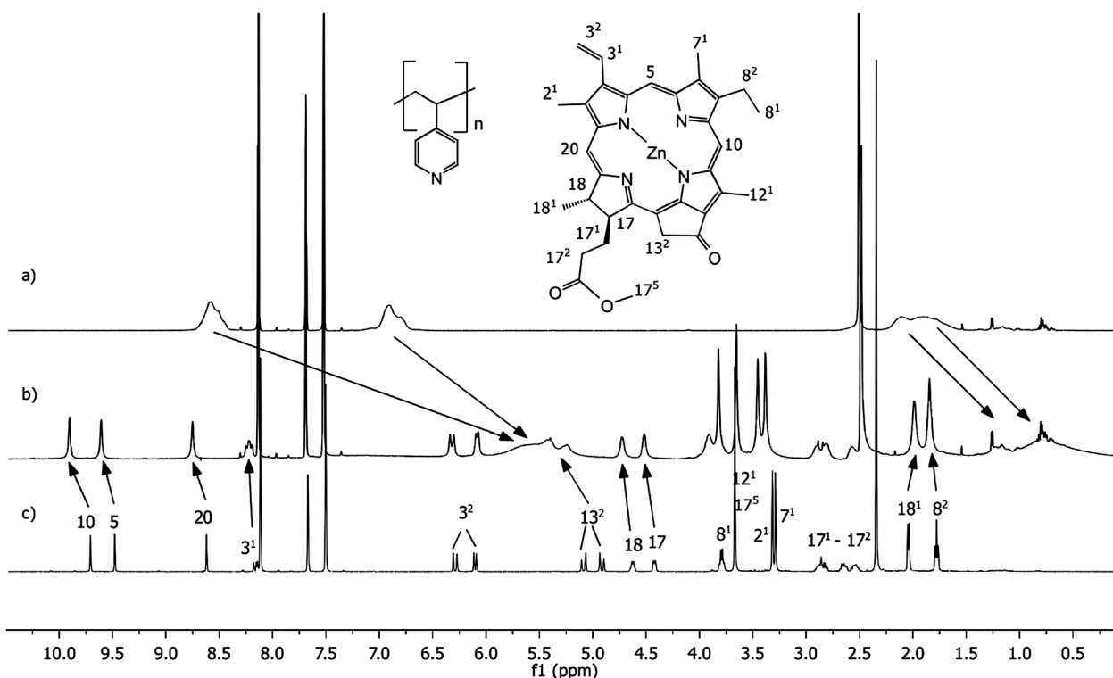
Fig. 3 1 H NMR spectra of (a) P4VP (polymer 52.6 μM; the molarity of pyridine units in the polymer backbone is 30 mM), (b) 1 : 3 mixture of ZnPPME (10 mM) and P4VP (polymer 52.6 μM; the molarity of pyridine units in the polymer backbone is 30 mM), (c) ZnPPME (10 mM) measured in d 5 -nitrobenzene.
