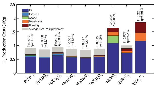
Fig. 5 Cost comparison of solar-hydrogen generators incorporating a 16% efficient PV component. The grey area represents the cost savings achieved by the improvements in PV efficiency. F and average solar to hydrogen efficiencies values ( \eta ) have been included for each system.
