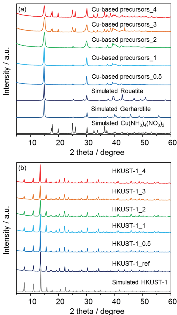
Fig. 3 XRD patterns of (a) the solvent insoluble Cu-based precursors (Cu-based precursors X ) with simulated patterns for Cu 2 (OH) 3 NO 3 (rouatite and gerhardtite) and Cu(NH 3 ) 4 (NO 3 ) 2 and (b) corresponding HKUST-1 X with HKUST-1 ref and simulated pattern for HKUST-1.
