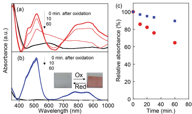
Fig. 3 In situ electrochemical UV spectra of (a) PVBPT and (b) PVPPP on ITO electrode. A neutral phenothiazine form was shown in black, and the corresponding radical cations under the applied potentials at 1.1 V were shown in red and blue, respectively. (c) Time decay of the relative absorbance at 518 nm ascribed to the radical cations for PVBPT (red) and PVPPP (blue).
