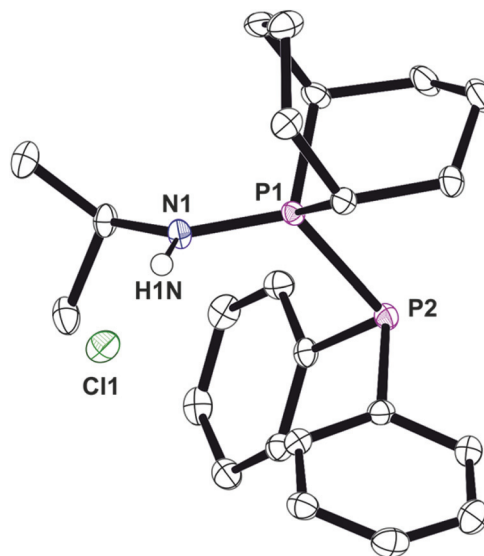
Fig. 7 Crystal structure of complex \mathbf{L}'_h \cdot \text{HCl} . All hydrogen atoms, except on the N1, have been omitted for clarity. Selected bond lengths (Å) and angles (°); P(1)–N(1) 1.6241(0), P(1)–P(2) 2.2403(4), N(1)–H(1N) 0.863(16), N(1)–P(1)–P(2) 119.93(4).
