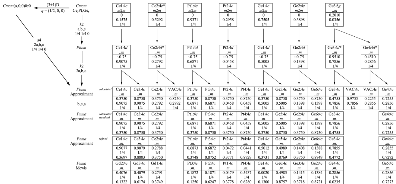
Fig. 5 Relation of the (3 + 1)D and 3D space groups of the modulated structure of Ce 3 Pt 4 Ge 6 . Group-supgroup scheme in the Bärnighausen formalism 40–43 for the subcell of Ce 3 Pt 4 Ge 6 (*occupancy parameter listed as 50% in the literature 24 ) and the supercell. The indices for the klassen-gleiche ( k ) symmetry reduction as well as the evolution of the atomic parameters are given. The index a is introduced for the formation of the approximant of the modulated structure. 39 The last line gives the atomic coordinates for Gd 3 Pt 4 Ge 6 , published by Mewis in space group Pnma . 25
