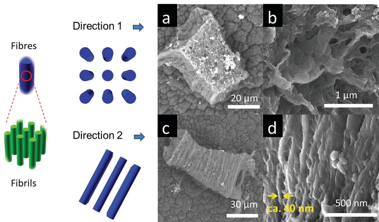
Fig. 3 PEDOT fibres (in blue) consists a bundle of fibrils (in green) that are formed in the MOF paralleled nano-channels. Since the PEDOT fibres are mostly aligned, SEM shows only rough surface in some orientations as (a) and (b), whereas it reveals aligned fibre-like morphology in other orientations as (c) and (d).
