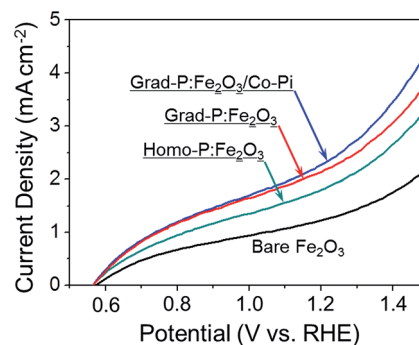
Fig. 7 I-V characteristics of bare \text{Fe}_2\text{O}_3 , homo-P: \text{Fe}_2\text{O}_3 , grad-P: \text{Fe}_2\text{O}_3 and grad-P: \text{Fe}_2\text{O}_3 /Co-Pi photoanodes measured for \text{H}_2\text{O}_2 oxidation under AM 1.5G illumination. The dark currents were negligible for all samples.
