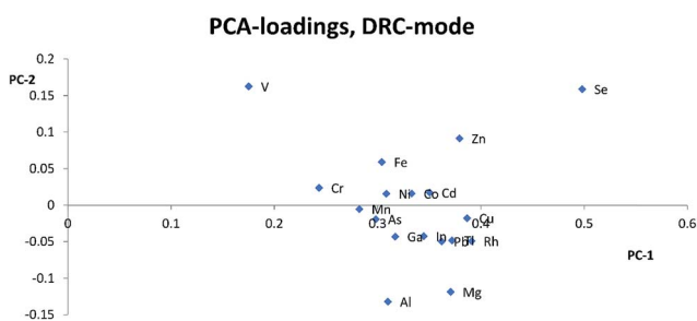
Fig. 3 Weighted PCA loadings according to explained variance including all matrixes in DRC-mode, based on centered \ln(x) transformed data for 24 Mg, 27 Al, 49 Ti, 51 V, 53 Cr, 55 Mn, 59 Co, 61 Ni, 65 Cu, 67 Zn, 69 Ga, 75 As, 82 Se, 103 Rh, 111 Cd, 115 In, 205 Tl, 208 Pb.
