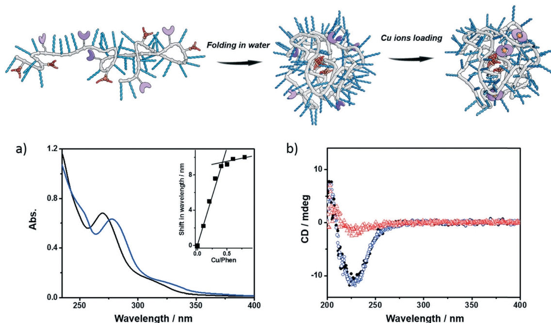
Fig. 2 Folding and Cu-loading of the polymers; a) UV-vis spectra of P1 (black, 0.6 mg mL -1 ) and P1@Cu(II) (blue, 0.6 mg mL -1 , [phen] : [Cu] = 2 : 1); b) CD spectra of P1 (0.5 mg mL -1 , black dot: 20 °C, red triangle: 90 °C), P1@Cu(II) (blue square, 20 °C, 0.5 mg mL -1 , [phen] : [Cu] = 2 : 1).
