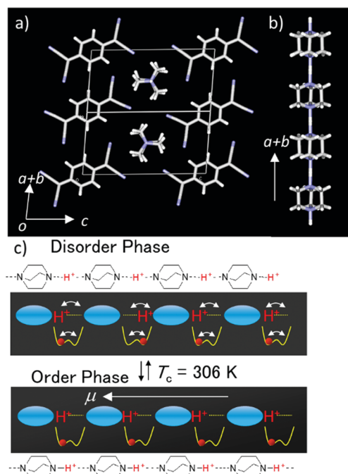
Fig. 3 Dynamic short-range collective proton transfer and dielectric switching in the organic semiconductor (\text{HDABCO}^+)\cdot(\text{TCNQ})_3 . (a) Unit cell viewed along the 1D (\text{N-H}^+\cdots\text{N})_\infty hydrogen-bonding chain and electrical conducting \pi -column of TCNQ. (b) High temperature 1D (\text{N-H}^+\cdots\text{N})_\infty hydrogen-bonding chain of \text{HDABCO}^+ cations along the a + b axis. Schematic potential energy curves of the \text{N-H}^+\cdots\text{N} hydrogen-bonding chain (c) at the high temperature paraelectric disordered phase (upper) and at the low temperature ordered ferroelectric phase (lower) for the proton orientation.
