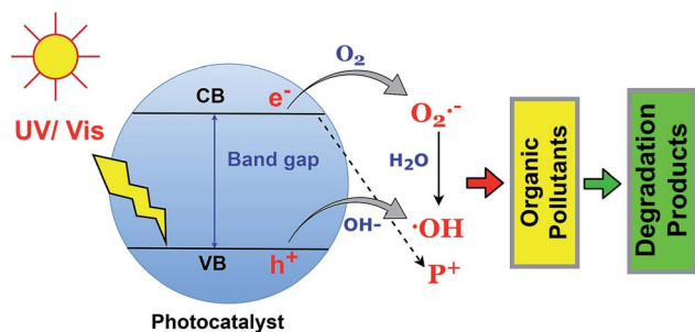
Fig. 6 Fundamentals of organic pollutant photodegradation by ROS.
