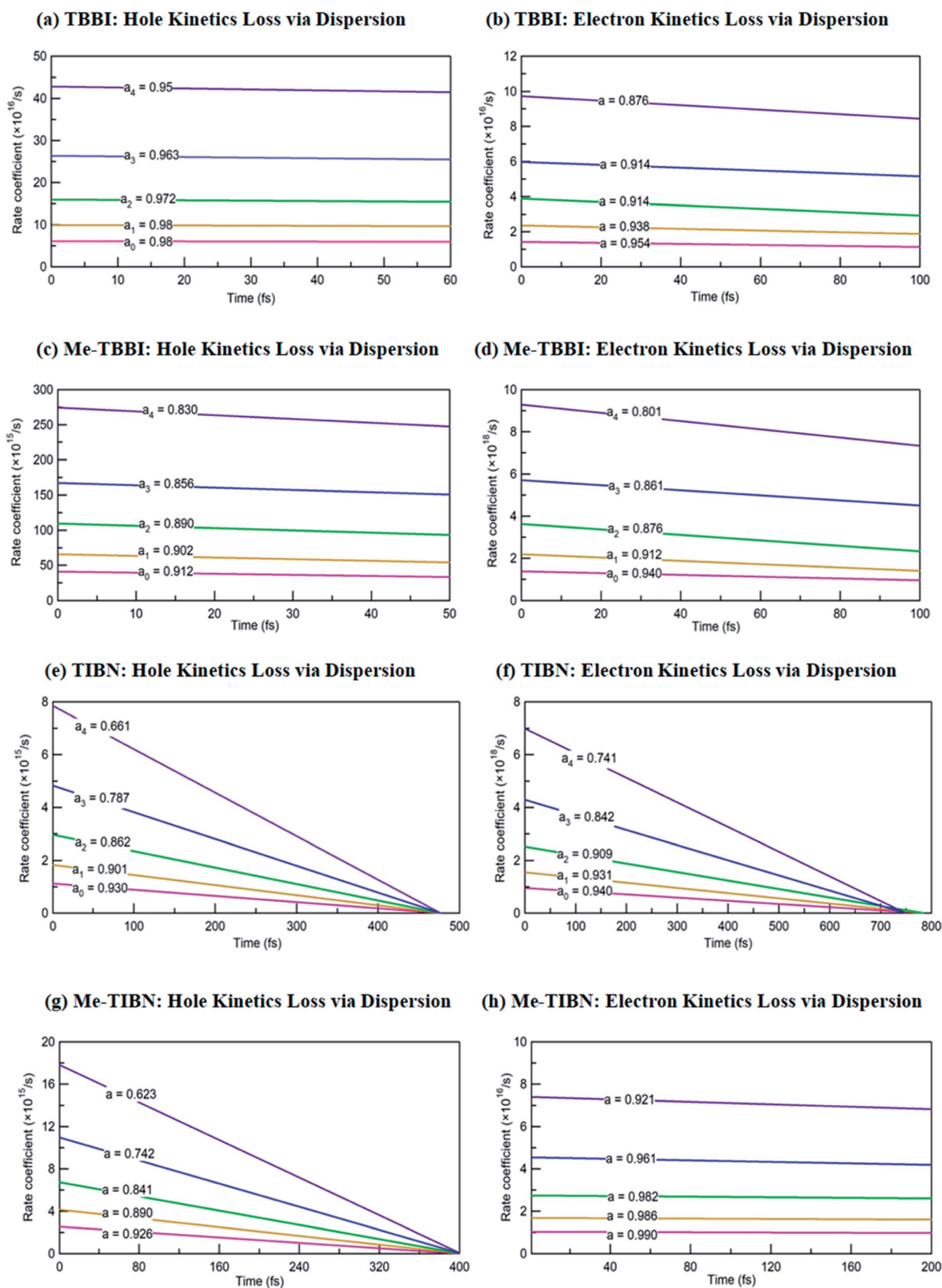
Fig. 6 The dispersive parameters ( a_0 , a_1 , a_2 , a_3 and a_4 ) at different applied fields of 0 , 7.144 \times 10^3 , 1.428 \times 10^4 , 2.143 \times 10^4 and 2.857 \times 10^4 V cm -1 for hole and electron transport in TBBI, Me-TBBI, TIBN and Me-TIBN molecules.
