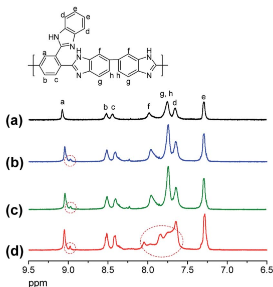
Fig. 5 1 H-NMR spectra of (a) pristine BIpPBI; (b) B20N5, (c) B20N10, and (d) BIpPBI after ex situ chemical stability test.
