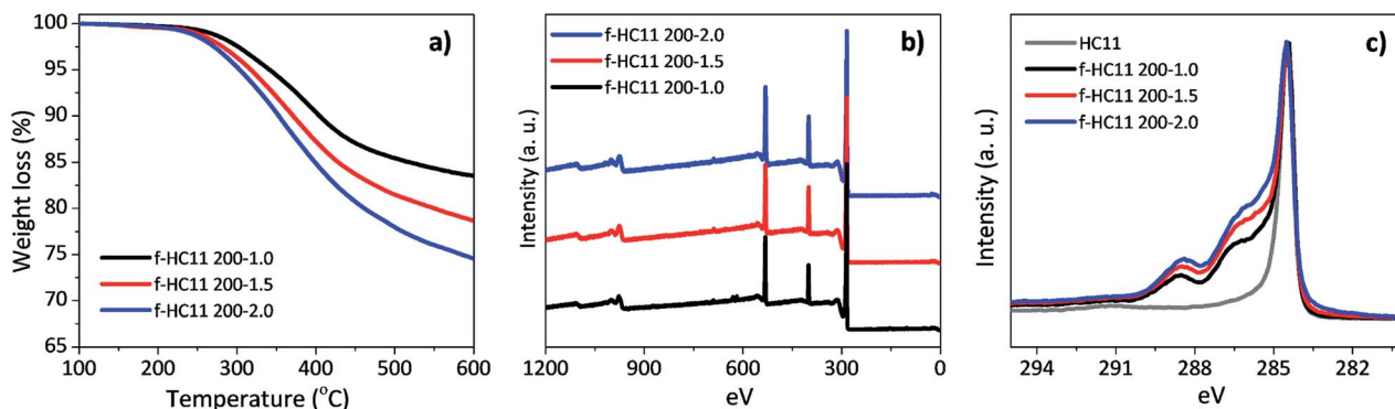
Fig. 8 (a) Thermogravimetric analysis, (b) XPS wide scan spectra, (c) high resolution C 1s spectra for the functionalized HC11 with different IDA weight ratios.
