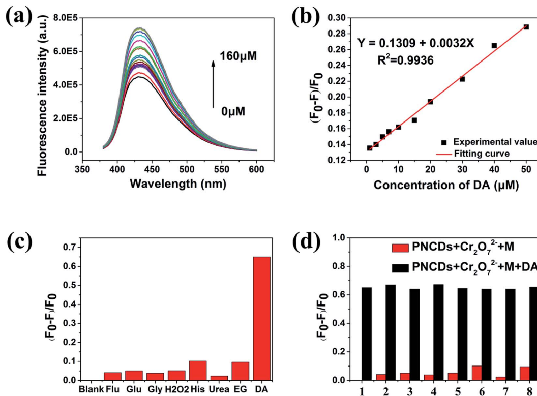
Fig. 5 (a) Fluorescence recovery of the PNCDs/ \text{Cr}(\text{vi}) mixture to DA at various concentrations (0, 0.5, 1, 3, 5, 7, 10, 15, 20, 30, 40, 50, 70, 90, 100, 120, 140, 150, 160 \mu\text{mol L}^{-1} ). (b) Plot of the (F_0 - F)/F_0 with the concentration of DA. (c) and (d) (F_0 - F)/F_0 of the PNCDs in PBS (pH: 7.4) with 160 \mu\text{M} different reducing biomolecules. F and F_0 correspond to the fluorescence intensities of the PNCDs without and with 160 \mu\text{M} of different reducing biomolecules (the numbers 1 to 8 are corresponding to blank, Flu, Glu, Gly, \text{H}_2\text{O}_2 , His, urea, EG, respectively).
