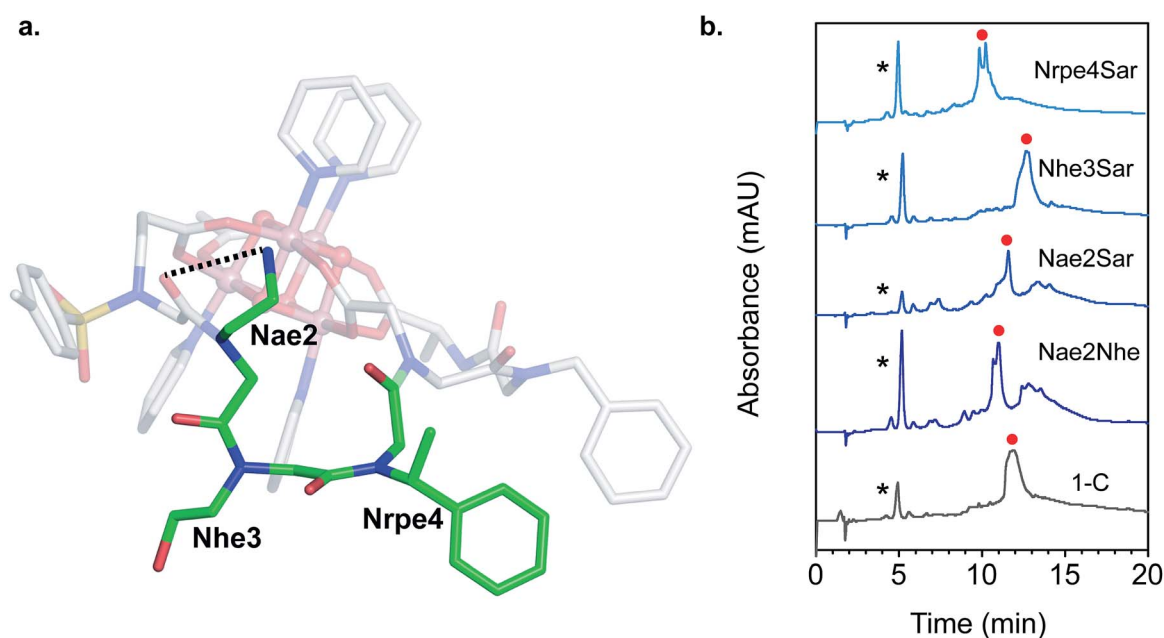
Fig. 6 (a) Close-up view of the loop region of 1-C. The loop residues are highlighted with green carbon atoms and labeled. The dashed line indicates the H-bond donor–acceptor distance. (b) LCMS of the crude reaction mixture between 1 and the mutated loop derivatives of H 3 C (both 0.5 mM) in methanol after 20 h at 50 °C. The asterisk (*) indicates residual 1 , and the red circle indicates peaks with masses corresponding to the hexadentate chelated cluster. Mobile phase: 5–95% gradient of acetonitrile/water with 10 mM NH 4 OAc/HOAc (pH ~ 5.2) buffer.
