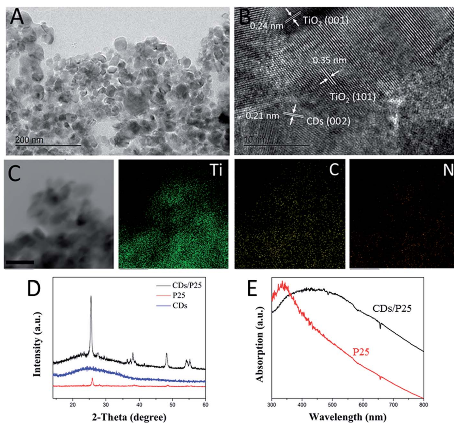
Fig. 1 (A) TEM image, (B) HRTEM image and (C) element mapping of CDs/TiO 2 nanocomposites, scale bar is 50 nm. (D) XRD patterns of P25, CDs and CDs/P25. (E) UV-vis spectrum of P25 and CDs/P25.
