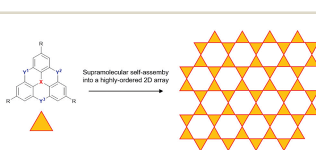
Fig. 29 Idealized schematic representation of the self-assembly of heteroatom-containing triangulenes into a supramolecular sheet-like array.
