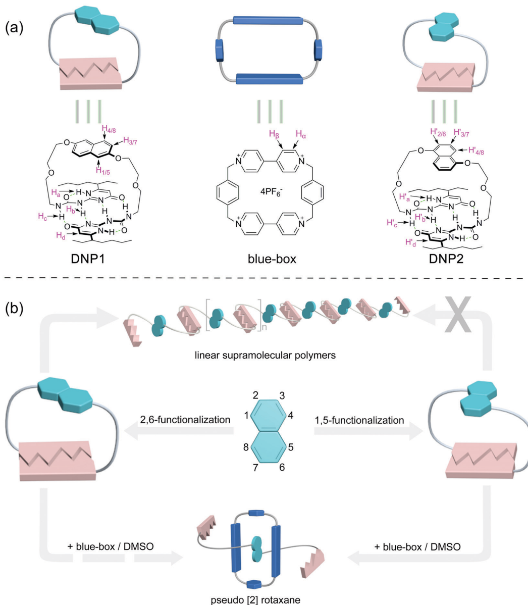
Fig. 1 (a) Chemical structures and cartoon representations of DNP1 , DNP2 , and the blue-box , and (b) schematic illustration of the supramolecular polymerizability of DNP1 and DNP2 , and their potential host-guest behaviors with the blue-box .
