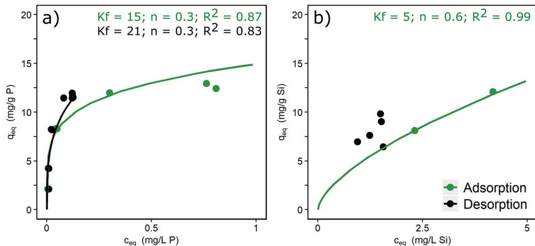
Fig. 2 Ad- and desorption isotherms for (a) phosphate ( c_0 = 3 \text{ mg L}^{-1} ) and (b) silicate ( c_0 = 10 \text{ mg L}^{-1} ) (pH 7.0, DI + NaCl) and Freundlich constants.
