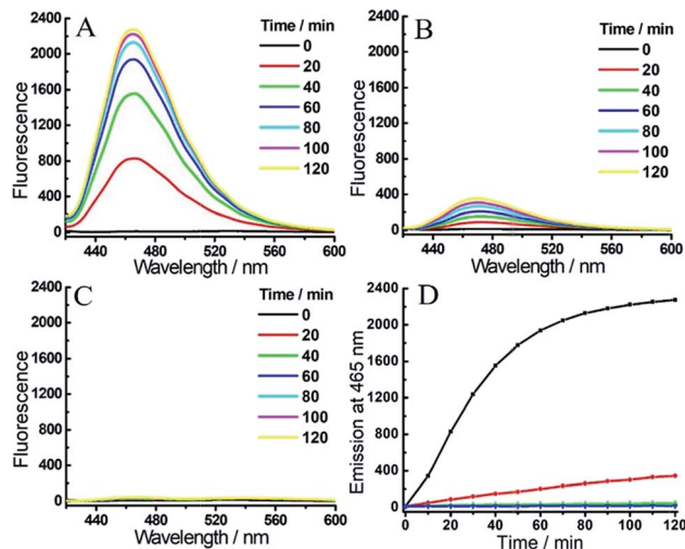
Fig. 2 Time-dependent fluorescent response of probe 1 ( 1 \mu\text{M} ) toward \text{H}_2\text{S} (200 \mu\text{M} ) and/or hNQO1 (1 \mu\text{g mL}^{-1} ). (A) 1 was treated with \text{H}_2\text{S} and hNQO1 simultaneously, or only with \text{H}_2\text{S} (B) or hNQO1 (C). (D) Time-dependent emissions at 465 nm for 1 treated with hNQO1 and \text{H}_2\text{S} (black), hNQO1 (green), \text{H}_2\text{S} (red) or probe 1 alone (blue) in PBS buffer.
