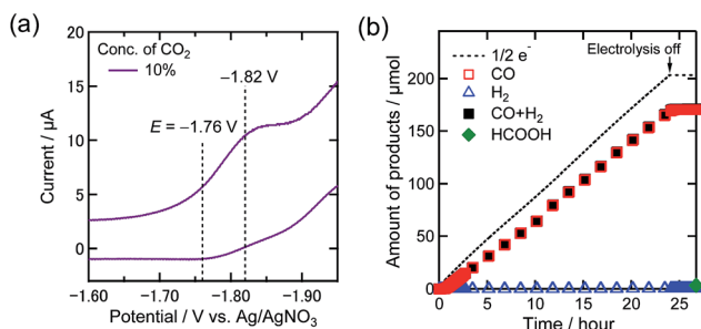
Fig. 5 (a) CV of the Re(I) complex (0.5 mM) in a DMF-TEOA mixed solution (5 : 1 v/v) containing Et 4 NBF 4 (0.1 M) under a 10% CO 2 atmosphere. Measurement conditions were the same as those in Fig. 3. (b) Time courses of the generation of CO (red square), H 2 (blue triangle), and formic acid (green diamond) with half of the electrons flowing (dotted line) during bulk electrolysis using the Re(I) catalyst (0.5 mM) at -1.76 V in a DMF-TEOA solution containing Et 4 NBF 4 (0.1 M) under a 10% CO 2 atmosphere (10 mL min -1 ).
