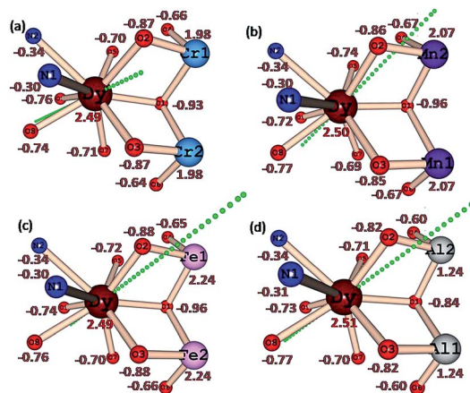
Fig. 8 Ab initio computed LoProp charges on the metal atoms and donor atoms of complexes (a) 1 \{\text{Cr}_2\text{Dy}_2\} , (b) 3 \{\text{Mn}_2\text{Dy}_2\} , (c) 5 \{\text{Fe}_2\text{Dy}_2\} and (d) 7 \{\text{Al}_2\text{Dy}_2\} (note: because of identical charges on the other half side, we have only shown here one side of the molecule).
