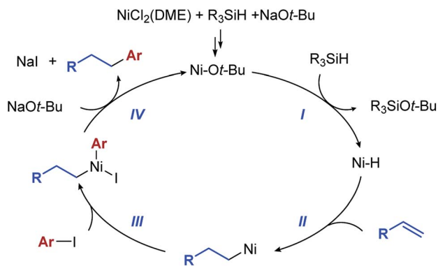
Scheme 3 Proposed mechanism of hydroarylation.
