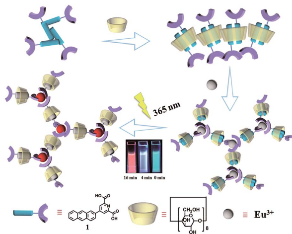
Fig. 1 Schematic illustration of the \gamma -cyclodextrin/anthracene/ \text{Eu}^{3+} supramolecular assembly and tunable lanthanide luminescence driven by reversible photo-cyclodimerization.
