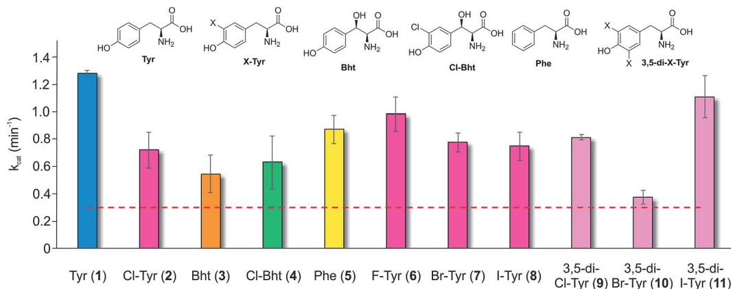
Fig. 3 Module 6 A-domain amino acid activation rates determined for the teicoplanin NRPS. Amino acids tested as substrates include tyrosine (1, blue), halogenated tyrosine residues (2 and 6–8, magenta), di-halogenated tyrosine residues (9–11, pale pink), Bht (orange, 3), Cl-Bht (green, 4) and phenylalanine (yellow, 5). Triplicate experiments, standard deviations indicated. Dotted line indicates the method detection limit.
