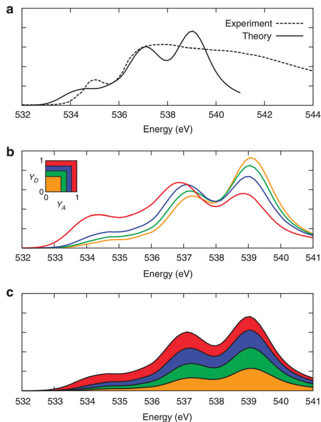
Fig. 8 XA spectra of liquid water. (a) Comparison of the calculated and experimental 28 XA spectra. (b) Calculated XA spectra of the four groups of molecules separated according to the asymmetry of their donor ( \gamma_D ) and acceptor ( \gamma_A ) environments, as shown in the inset. (c) Contributions of the four groups into the total XA spectrum. The colour coding is shown in the inset above. Reproduced from ref. 13.
