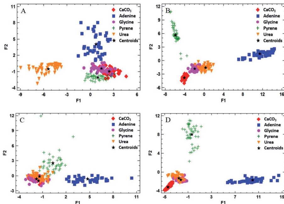
Fig. 5 DFA of the doped matrix samples with organic compounds using C(i), H(i), O(i) and N(i) emission lines besides CN and C 2 emission bands as input quantitative variables. The experiment was carried out at 7 mb pressure and using 72.4 J cm -2 as the fluence value, firing sets of 25 single laser shots in 3 different fresh sampling positions in the atmosphere of (A) CO 2 , 10 wt% organic dopant; (B) CO 2 , 50 wt% organic dopant; (C) air, 10 wt% organic dopant; (D) air, 50 wt% organic dopant.
