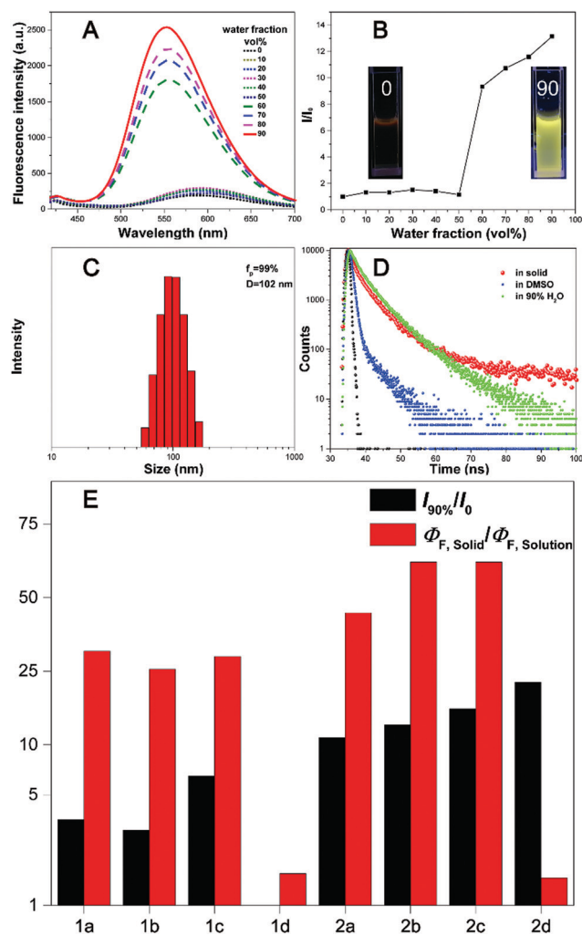
Fig. 4 (A) Fluorescence spectra of 2b in DMSO/water with different water fractions. (B) The I_{90}/I_0 ratios of 2b in DMSO/water with different water fractions. (C) Particle size distribution of 2b in a DMSO/water mixture with an f_p value of 99%. (D) Emission decay of 2b in DMSO, H 2 O, and the solid state. (E) Ratio of the quantum yields for the solid and solution states of all compounds, and the ratio of the fluorescence intensity in the aggregation and solution states.
