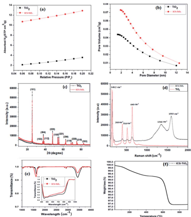
Fig. 3 (a) Nitrogen adsorption/desorption isotherms; (b) nitrogen desorption/desorption pore size distribution; (c) XRD pattern, (d) Raman spectra; (e) FTIR spectra of \text{TiO}_2 and ICS- \text{TiO}_2 ; (f) TGA of ICS- \text{TiO}_2 .
