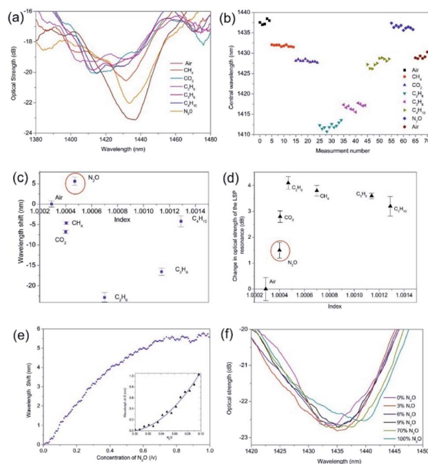
Fig. 7 The typical experimental results of a UV processed Ge/SiO 2 /Pt LSP fibre device coated with SWNTs and PEI as a function of surrounding refractive index and the detection of nitrous oxide (a) the transmission spectra as function of changing surrounding index and the nitrous oxide. (b) The individual measurements of the central wavelength of the LSP resonance for each alkane gas and nitrous oxide (c) and (d) the wavelength and optical strength sensitivity as a function of the different gases and their refractive index respectively. (e) The wavelength response to increasing N_2O concentration, the insert showing the wavelength shift with low concentrations of N_2O . (f) Examples of the changes in transmission spectra of LSP resonance to various concentrations of N_2O as a percentage of total volume.
