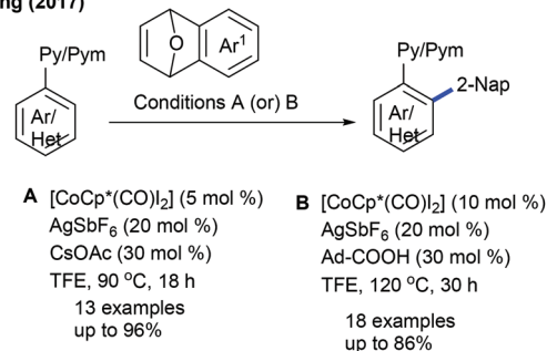
Scheme 22 Addition of arenes with oxabenzonorbornadienes.
