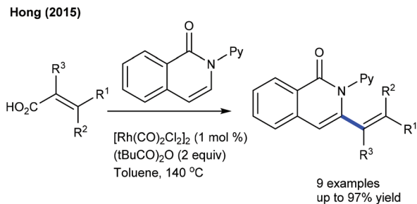
Scheme 32 Decarboxylative C–H alkenylation of quinolones/isoquinolones.
