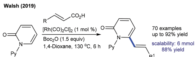
Scheme 33 Decarboxylative C–H alkenylation of pyridones.
