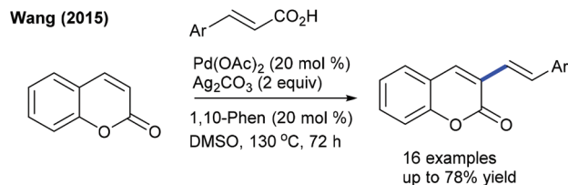
Scheme 36 C3-Alkenylation of coumarins via decarboxylative cross-coupling.
