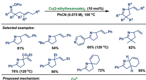
Scheme 5 Bower's copper-catalyzed Heck-like cyclizations of \gamma,\delta -unsaturated oxime esters.
