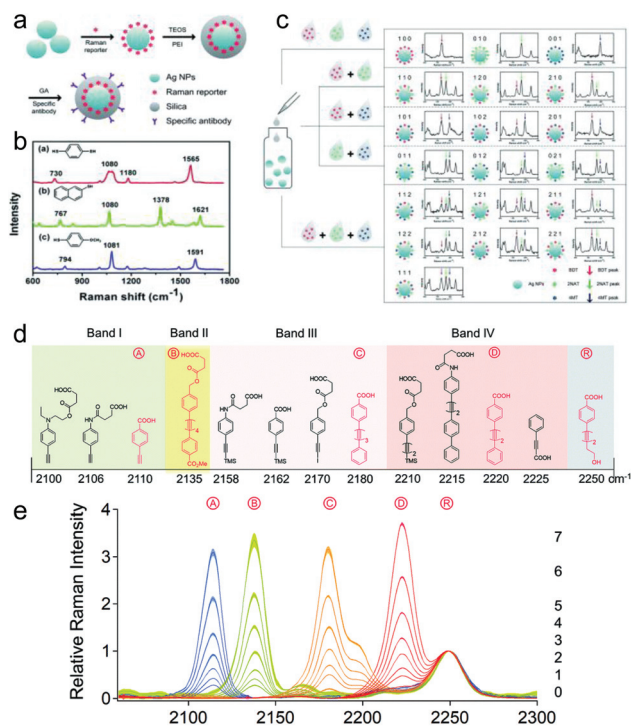
Fig. 7 (a) Schematic illustration of the preparation of the encoded SERS nanoprobe. Silver nanoparticles were used as the SERS-active substrates, on which Raman reporters were adsorbed as the coding agents. Then, a layer of silica shell was coated for both protecting Raman reporters from the surroundings and providing a platform for further surface modifications. (b) SERS spectra of three SERS nanoprobe and the chemical structures of encoded Raman reporters: BDT, 2-NAT and 4-MT. (c) Codes, structures, and measured spectra of the synthesized 19 SERS encoders. The spectra are only shown from wavenumber 600 to 900 for clarity. (d) Molecular structures and Raman spectral properties of alkyne candidates for super-capacity coding systems. They are categorized into 4 spectral bands: bands I, II, III, and IV. Experimentally, these compounds labeled with \textcircled{A} , \textcircled{B} , \textcircled{C} , \textcircled{D} , and \textcircled{E} were selected to covalently attach to aminolated resin beads. (e) Eight Raman codes generated through mixing the compounds with different amount ratios. They correspond to \textcircled{A}_n ( n = 0-7 ) at 2110 \text{ cm}^{-1} , \textcircled{B}_n ( n = 0-7 ) at 2135 \text{ cm}^{-1} , \textcircled{C}_n ( n = 0-7 ) at 2180 \text{ cm}^{-1} , and \textcircled{D}_n ( n = 0-7 ) at 2220 \text{ cm}^{-1} , respectively. (a-c) Reproduced with permission from ref. 39. Copyright 2014, Royal Society of Chemistry. (d and e) Reproduced with permission from ref. 41. Copyright 2020, Royal Society of Chemistry.
